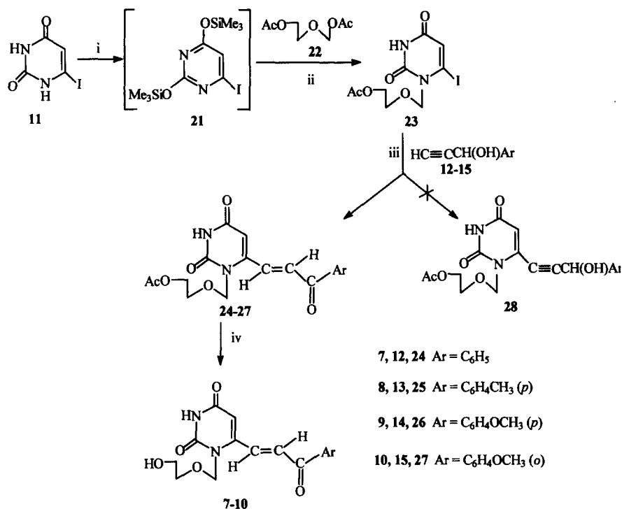
Scheme 2. Reaction conditions: (i) HMDS, TMSCl, bz, reflux, 4–6h; (ii) 1,2-dichloroethane, SnCl 4 , rt, overnight; (iii) (PPh 3 ) 2 , PdCl 2 , CuI, Et 3 N, DMF, 55°C, 6h, N 2 ; (iv) NaOMe, MeOH, rt, 4h.
