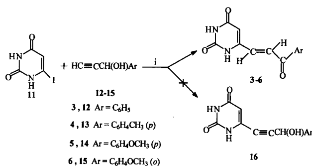
Scheme 1. Reaction condition: (i) (PPh 3 ) 2 PdCl 2 , CuI, Et 3 N, DMF, 55 °C, 6 h.
